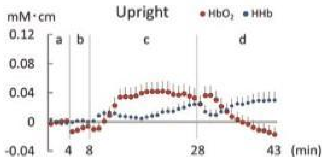
Fig. 1 Temporal changes in the averaged oxyhaemoglobin (HbO 2 ) and deoxyhaemoglobin (HHb) levels in the right prefrontal cortex during cycling in the upright and supine positions. (a) Pre-exercise rest. (b) Warm-up. (c)
